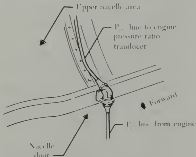
FIGURE 8-15. Turbine discharge pressure ( P_7 ) pickup.
